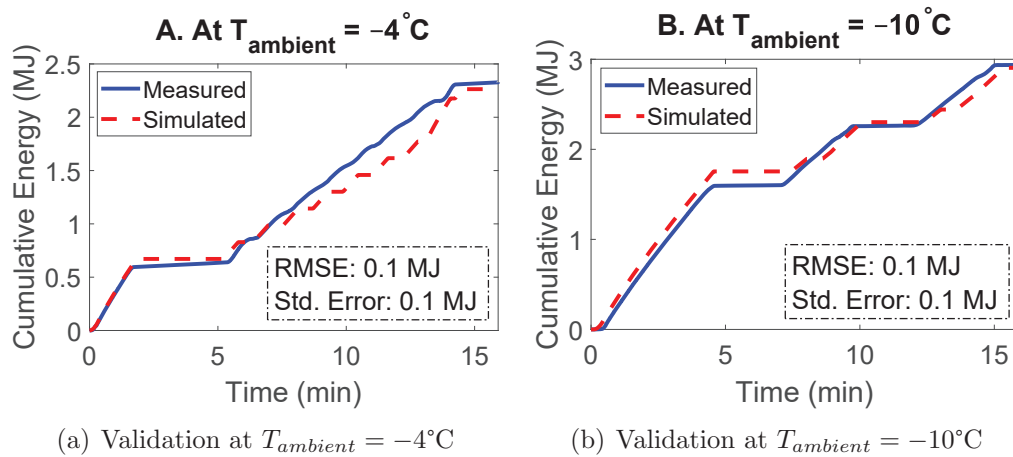
Figure 4.11: Validation of cabin electric heater energy consumption
