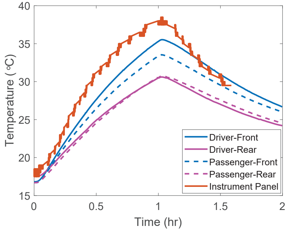
Figure 4.3: Temperature distribution inside test vehicle cabin
